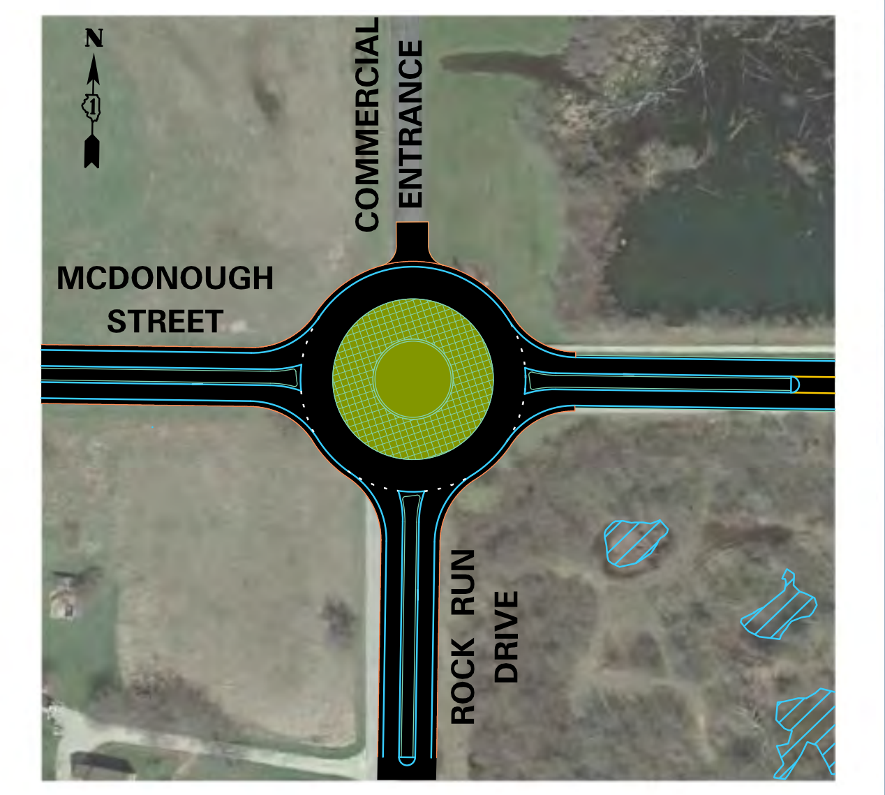
MCDONOUGH ST / ROCK RUN DRIVE ROUNDBOUT INTERSECTION ALTERNATIVE ALTERNATIVE EW-1B
